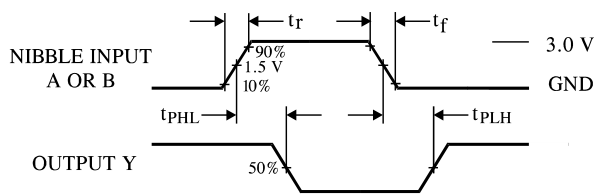
Figure 1. Switching Waveforms
