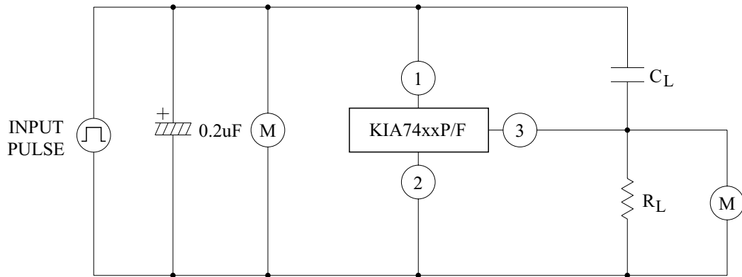
TEST CIRCUIT 2.
