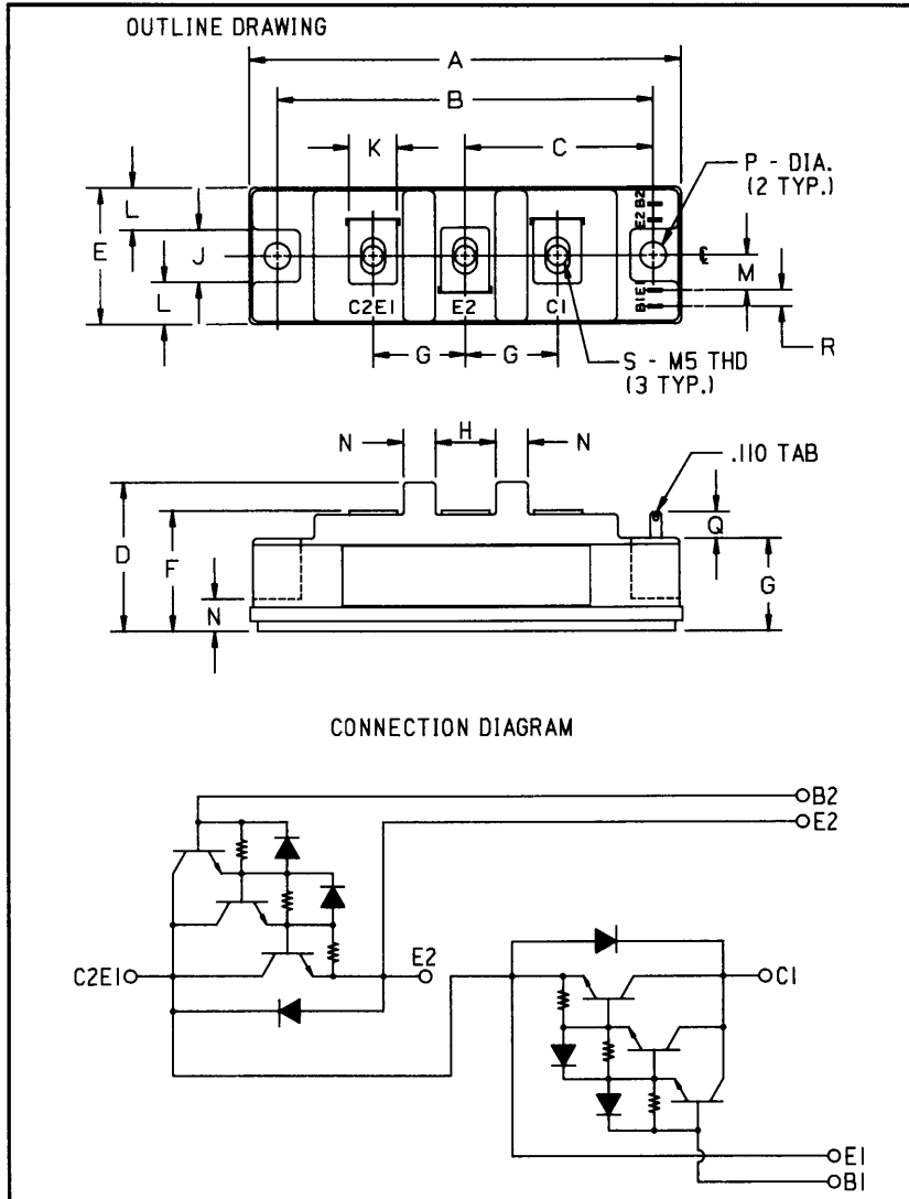
Outline Drawing
