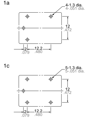
PC board pattern (Copper-side view)
