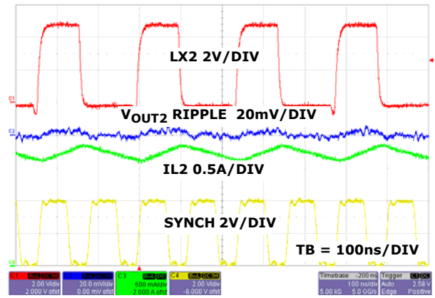
FIGURE 34. STEADY STATE OPERATION AT FULL LOAD (PFM) WITH FREQUENCY = 8MHz CHANNEL 2
