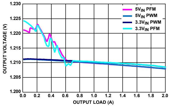
FIGURE 13. V_{OUT} REGULATION vs LOAD, F_{SW} = 2\text{MHz} , V_{OUT} = 1.2\text{V} , T_A = +25^\circ\text{C}
