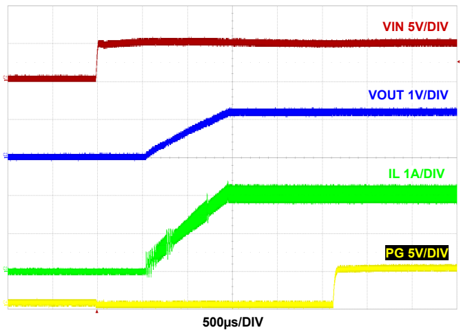
FIGURE 31. START-UP V_{IN} AT 2A LOAD F_{SW} = 2\text{MHz} , V_{IN} = 5\text{V} , MODE = PWM, T_A = +25^\circ\text{C}
