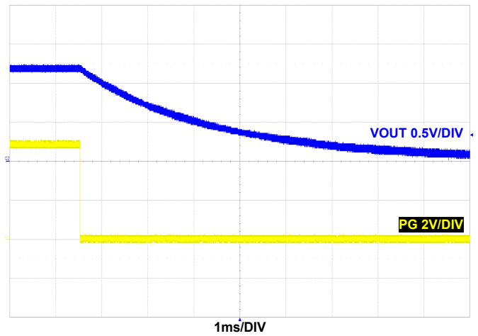
FIGURE 49. OVER-TEMPERATURE PROTECTION F_{SW} = 2\text{MHz} , V_{IN} = 5\text{V} , MODE = PWM, T_A = +163^\circ\text{C}
