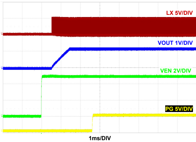
FIGURE 22. START-UP AT 2A LOAD F_{SW} = 2\text{MHz} , V_{IN} = 5\text{V} , MODE = PWM, T_A = +25^\circ\text{C}
