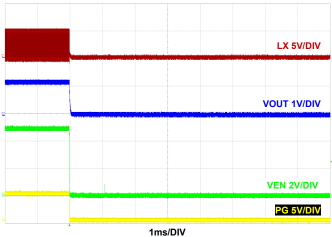
FIGURE 25. SHUTDOWN AT 2A LOAD F_{SW} = 2\text{MHz} , V_{IN} = 5\text{V} , MODE = PFM, T_A = +25^\circ\text{C}
