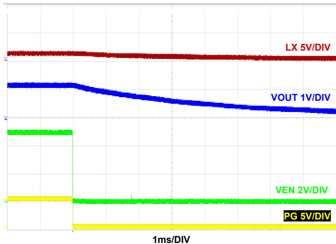
FIGURE 20. SHUTDOWN AT NO LOAD F_{SW} = 2\text{MHz} , V_{IN} = 5\text{V} , MODE = PFM, T_A = +25^\circ\text{C}
