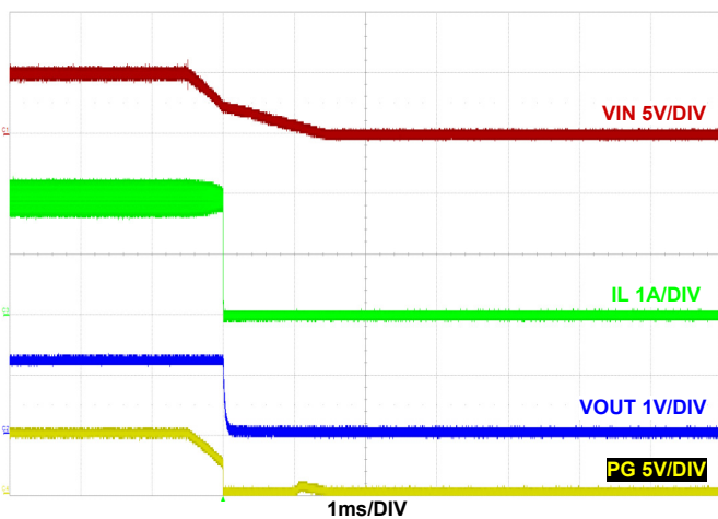
FIGURE 32. SHUTDOWN V_{IN} AT 2A LOAD F_{SW} = 2\text{MHz} , V_{IN} = 5\text{V} , MODE = PFM, T_A = +25^\circ\text{C}
