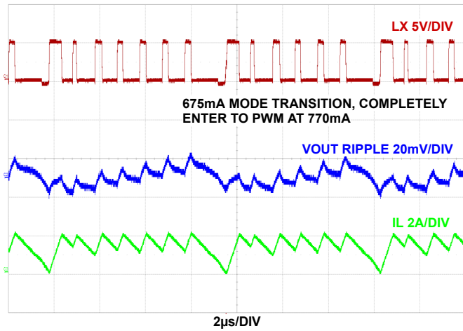
FIGURE 46. PFM TO PWM TRANSITION F_{SW} = 2\text{MHz} , V_{IN} = 5\text{V} , MODE = PFM, T_A = +25^\circ\text{C}
