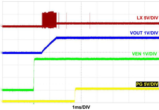
FIGURE 18. START-UP AT NO LOAD F_{SW} = 2\text{MHz} , V_{IN} = 5\text{V} , MODE = PFM, T_A = +25^\circ\text{C}
