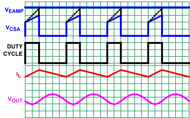
FIGURE 50. PWM OPERATION WAVEFORMS
