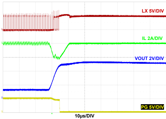
FIGURE 48. OVERVOLTAGE PROTECTION F_{SW} = 2\text{MHz} , V_{IN} = 5\text{V} , MODE = PFM, T_A = +25^\circ\text{C}
