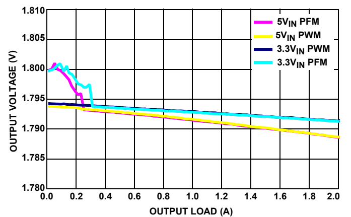
FIGURE 15. V_{OUT} REGULATION vs LOAD, F_{SW} = 2\text{MHz} , V_{OUT} = 1.8\text{V} , T_A = +25^\circ\text{C}
