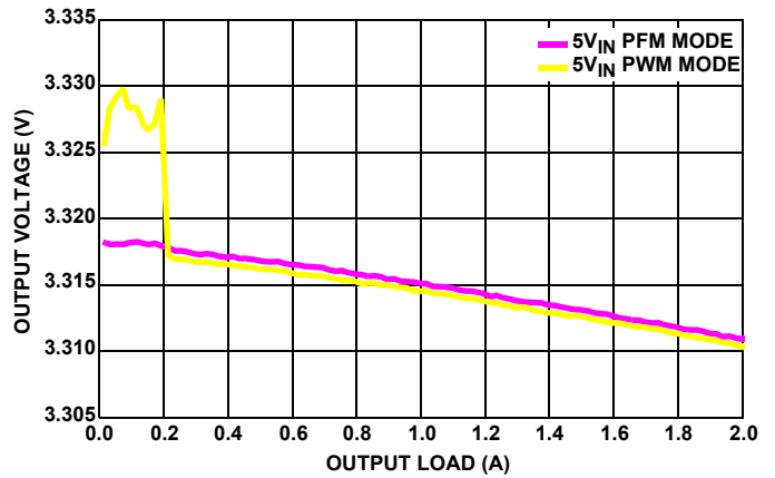
FIGURE 17. V_{OUT} REGULATION vs LOAD, F_{SW} = 2\text{MHz} , V_{OUT} = 3.3\text{V} , T_A = +25^\circ\text{C}
