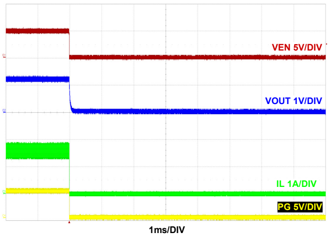
FIGURE 29. SHUTDOWN AT 1.5A LOAD F_{SW} = 2\text{MHz} , V_{IN} = 5\text{V} , MODE = PFM, T_A = +25^\circ\text{C}
