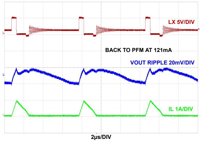
FIGURE 47. PWM TO PFM TRANSITION F_{SW} = 2\text{MHz} , V_{IN} = 5\text{V} , MODE = PWM, T_A = +25^\circ\text{C}
