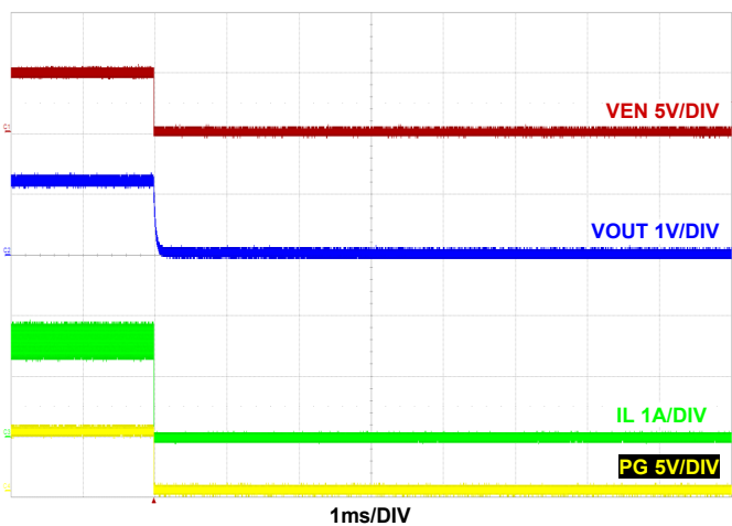
FIGURE 27. SHUTDOWN AT 1.5A LOAD F_{SW} = 2\text{MHz} , V_{IN} = 5\text{V} , MODE = PWM, T_A = +25^\circ\text{C}
