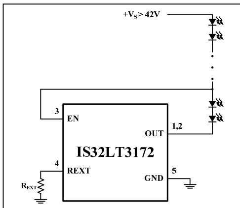
Figure 38 High Input Voltage Application Circuit
