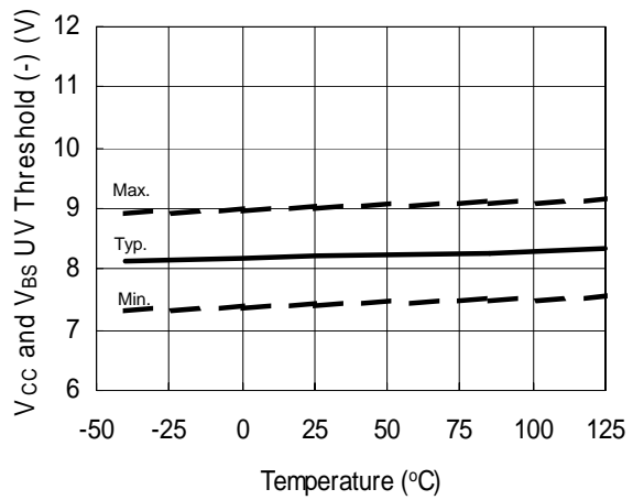
Figure 18. V_{CC} and V_{BS} Undervoltage Threshold (-) vs. Temperature
