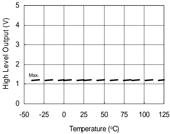
Figure 10A. High Level Output vs. Temperature
