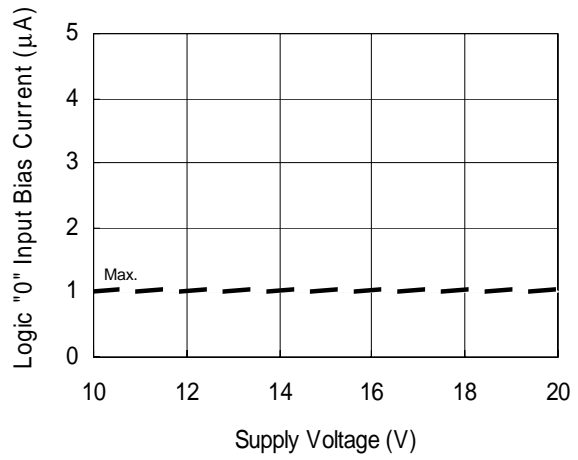
Figure 16B. Logic "0" Input Bias Current vs. Supply Voltage
