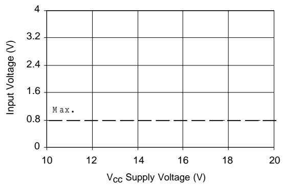
Figure 13B. Logic "0" (HO) & Logic "1" (LO) & Active SD Input Voltage vs. Supply Voltage
