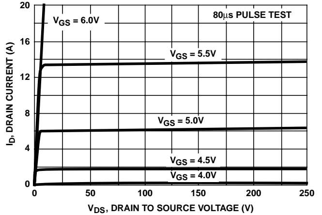
FIGURE 5. OUTPUT CHARACTERISTICS
