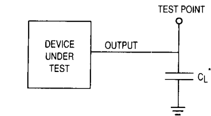
Figure 5. Test Circuit
