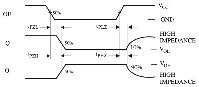
Figure 2. Switching Waveforms
