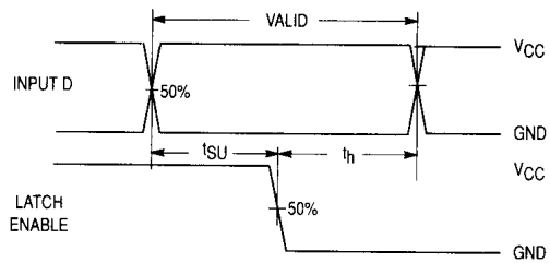
Figure 2. Switching Waveforms
