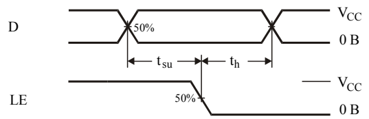
Figure 4. Switching Waveforms
