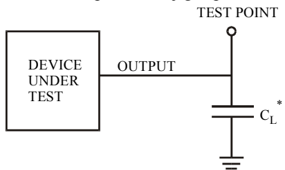
Figure 5. Test Circuit
