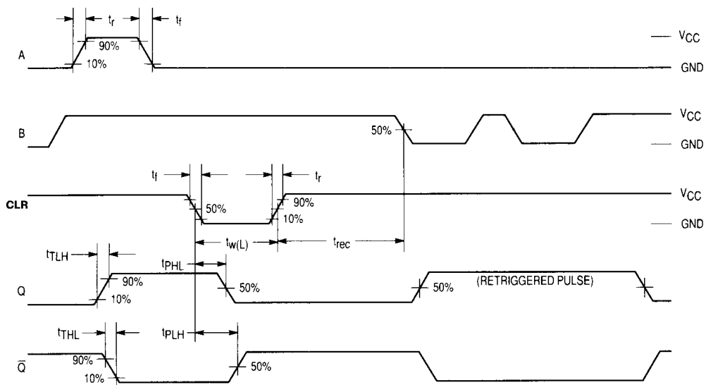
Figure 2. Switching Waveforms
