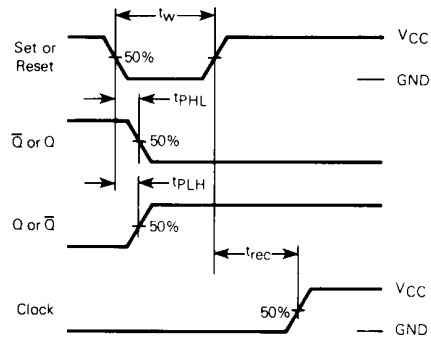
Figure 2. Switching Waveforms
