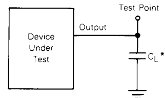
Figure 4. Test Circuit
