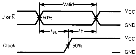
Figure 3. Switching Waveforms
