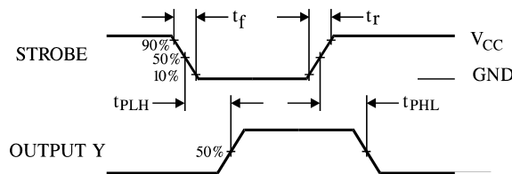
Figure 4. Switching Waveforms
