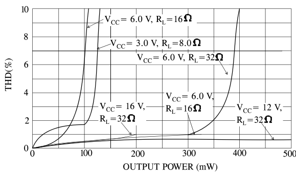
Figure 5. DISTORTION versus POWER f = 1.0 kHz, AVD = 34 dB
