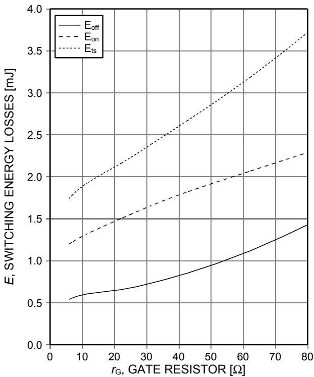
Figure 13. Typical switching energy losses as a function of gate resistor (inductive load, T_{vj}=175^{\circ}\text{C} , V_{CE}=400\text{V} , V_{GE}=15/0\text{V} , I_C=40\text{A} , Dynamic test circuit in Figure E)
