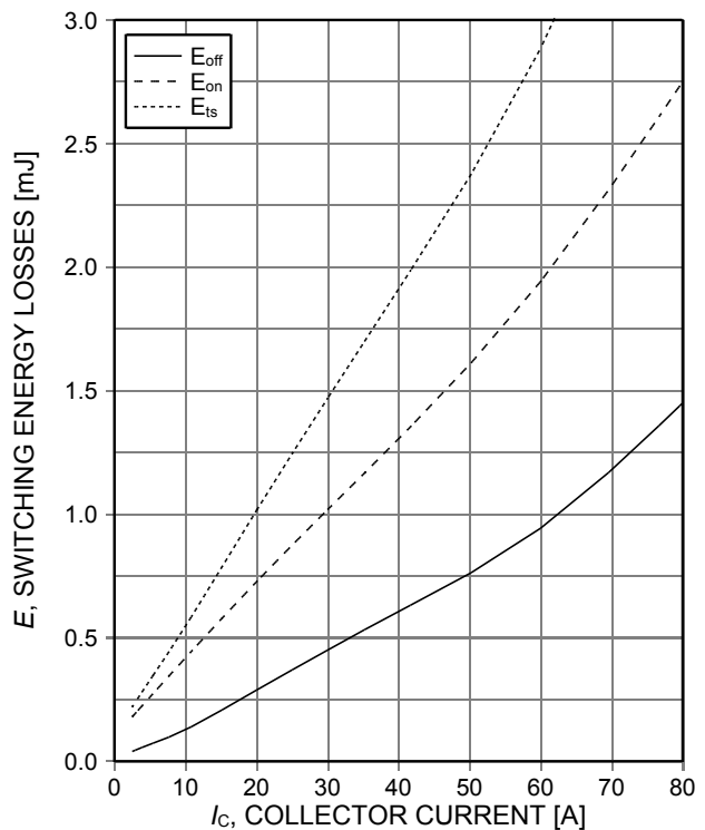
Figure 12. Typical switching energy losses as a function of collector current (inductive load, T_{vj}=175^{\circ}\text{C} , V_{CE}=400\text{V} , V_{GE}=15/0\text{V} , r_G=10\Omega , Dynamic test circuit in Figure E)
