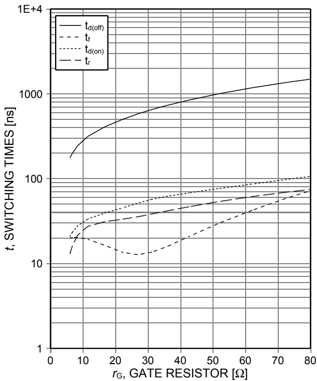
Figure 9. Typical switching times as a function of gate resistor (inductive load, T_{vj}=175^{\circ}\text{C} , V_{CE}=400\text{V} , V_{GE}=15/0\text{V} , I_C=40\text{A} , Dynamic test circuit in Figure E)
