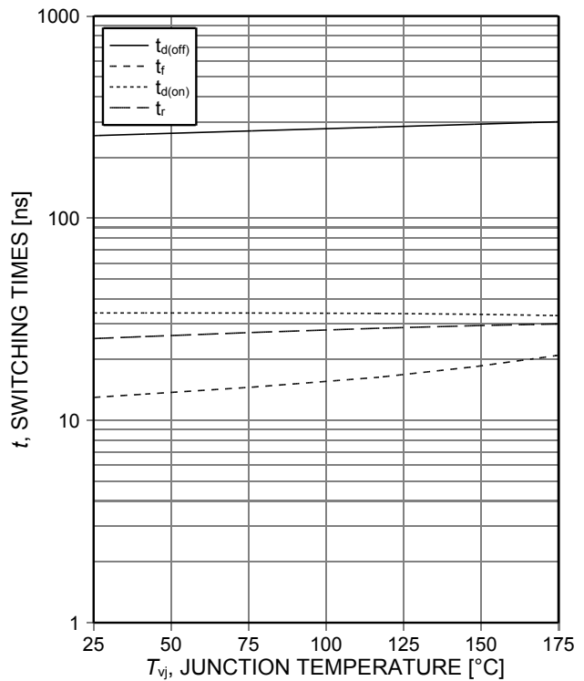
Figure 10. Typical switching times as a function of junction temperature (inductive load, V_{CE}=400\text{V} , V_{GE}=15/0\text{V} , I_C=40\text{A} , r_G=10\Omega , Dynamic test circuit in Figure E)
