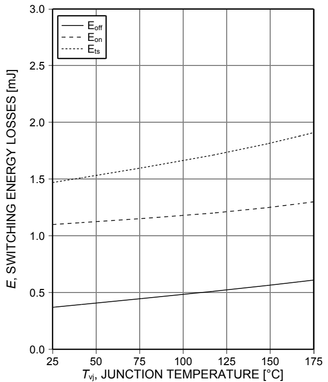
Figure 14. Typical switching energy losses as a function of junction temperature (inductive load, V_{CE}=400\text{V} , V_{GE}=15/0\text{V} , I_C=40\text{A} , r_G=10\Omega , Dynamic test circuit in Figure E)
