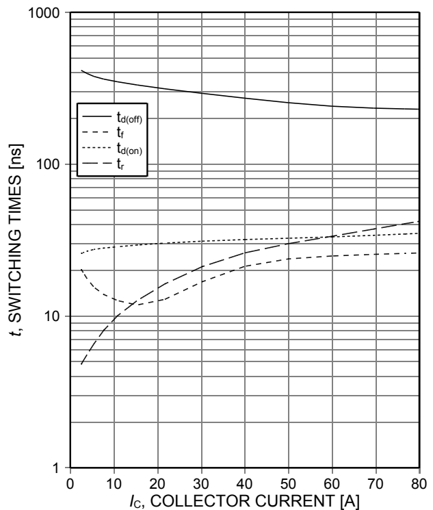
Figure 8. Typical switching times as a function of collector current (inductive load, T_{vj}=175^{\circ}\text{C} , V_{CE}=400\text{V} , V_{GE}=15/0\text{V} , r_G=10\Omega , Dynamic test circuit in Figure E)
