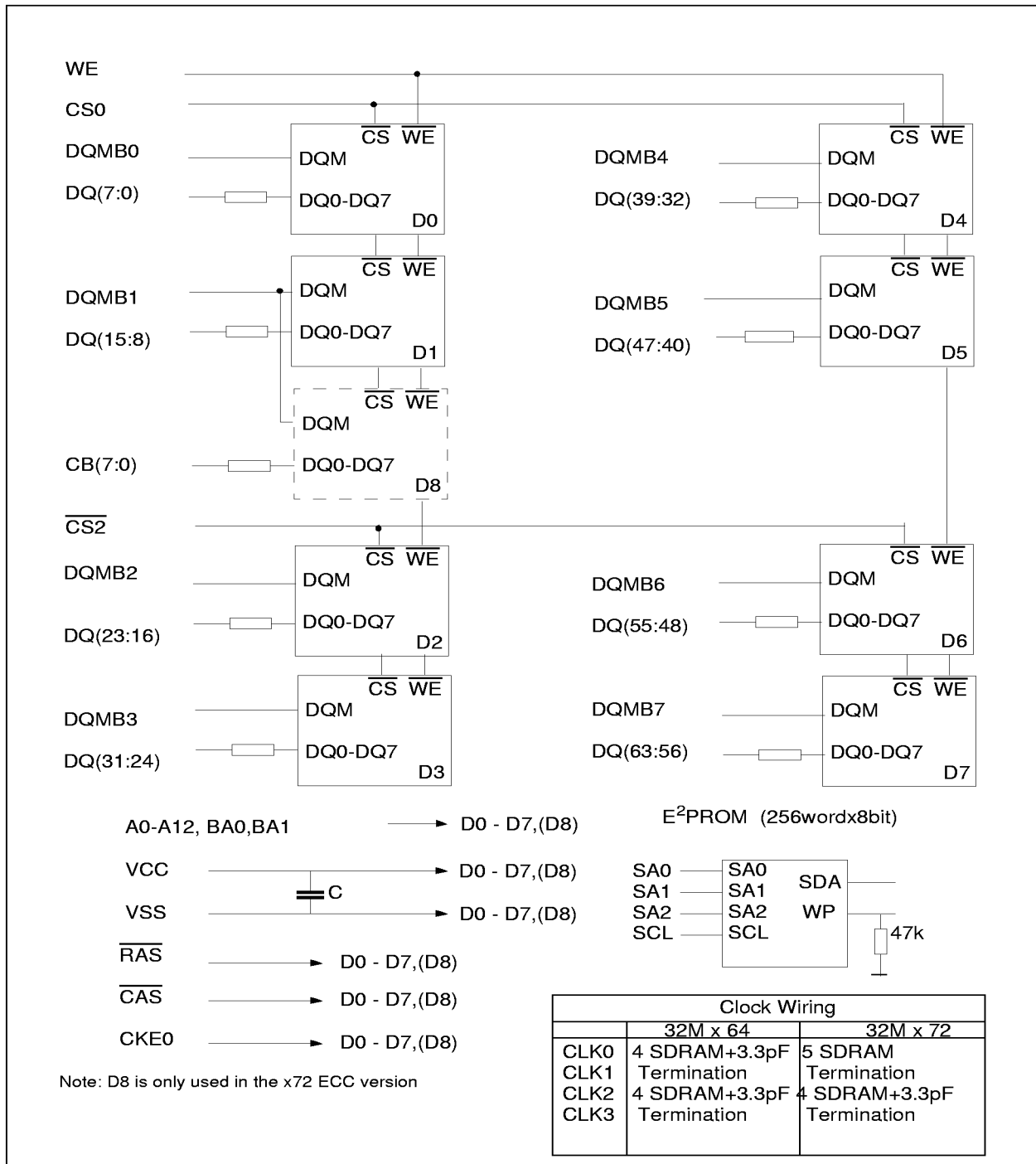
Block Diagram for 32M x 64/72 one bank SDRAM DIMM modules
