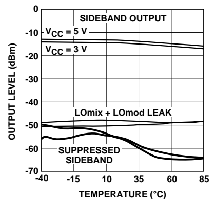
Figure 15. Modulator + Mixer SSB Output Levels vs. Temperature and V_{CC} .
