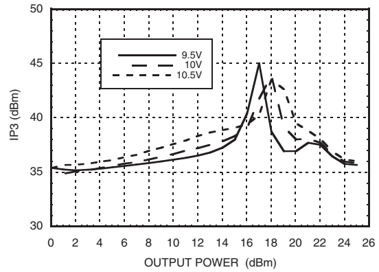
Output IP3 vs. Output Power
