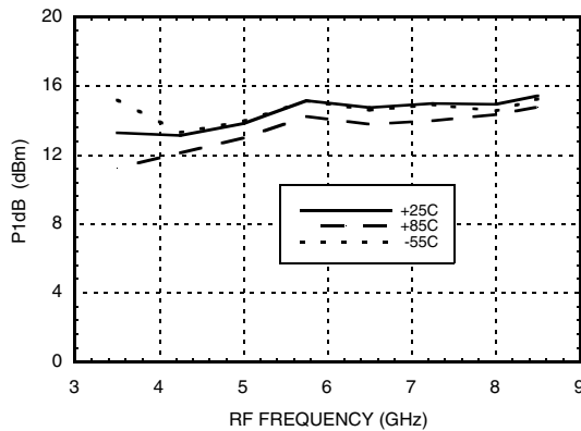
Input P1dB vs. Temperature
