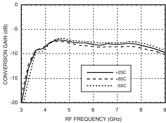
Conversion Gain vs. Temperature
