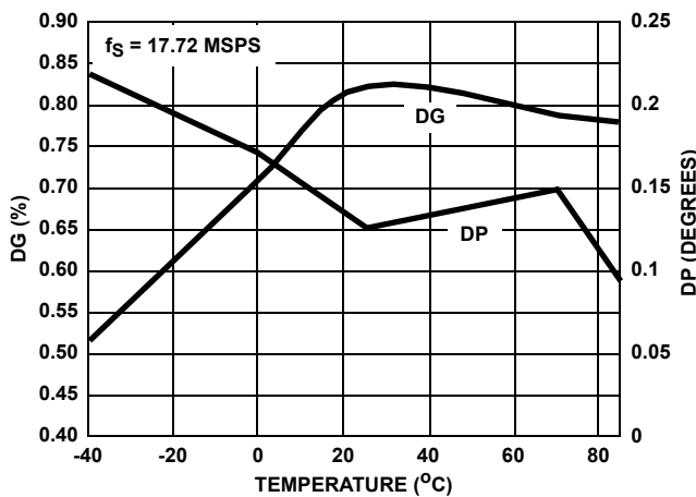
FIGURE 19. DIFFERENTIAL GAIN/PHASE vs TEMPERATURE
