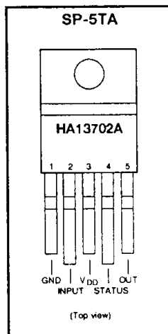
Figure 1 Pin Arrangement
