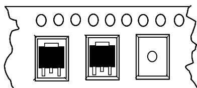
Feed Direction TO252 - 263 Package Orientation
