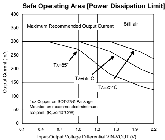
Note: V_{IN(max)} \leq 5.5V Figure 2. Safe Operating Area
