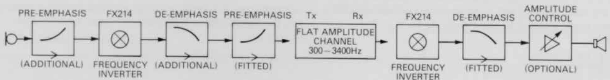
Fig. 4 Recommended Basic Radio Communication Audio System Layout
