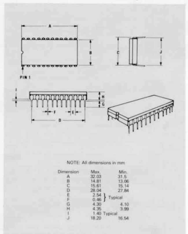
Fig. 9 FX224J 24-pin DIL Package
