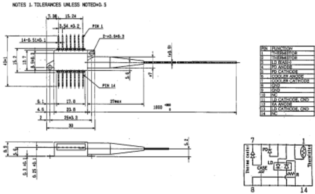
FU-632SEA-3MxxA/FU-632SEA-6MxxA
