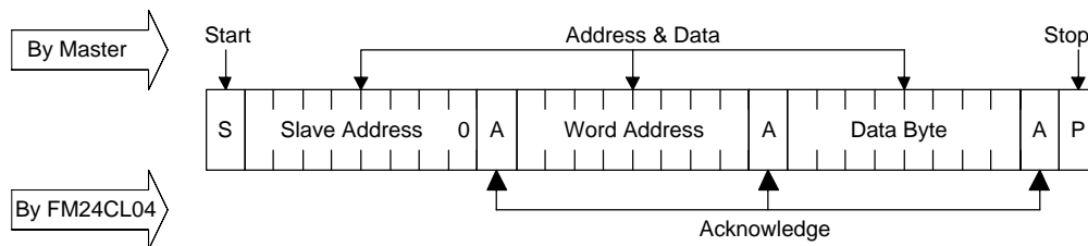
Figure 5. Byte Write
