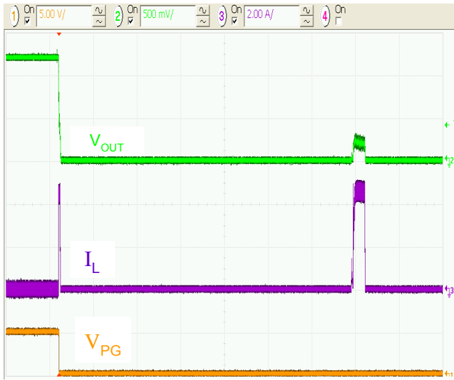
Figure 26. V OUT to GND Short Circuit, 200μs/div.
