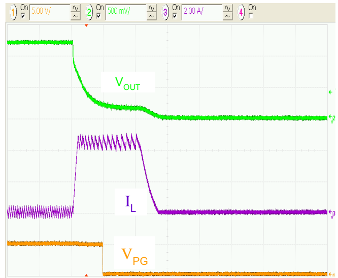
Figure 27. V OUT to GND Short Circuit, 5μs/div.
