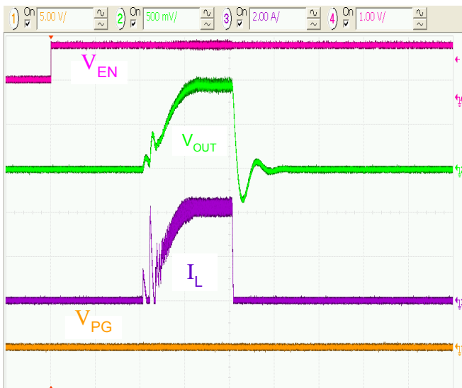
Figure 28. Over-Current at Startup, R_{LOAD}=200m\Omega , 50μs/div.
