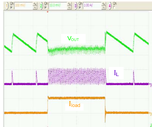
Figure 19. 24mA to 500mA to 24mA, MODE=0, 5 \mu s /div.
