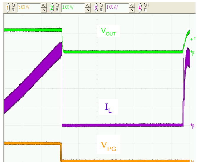
Figure 29. Progressive Overload, 200μs/div.
