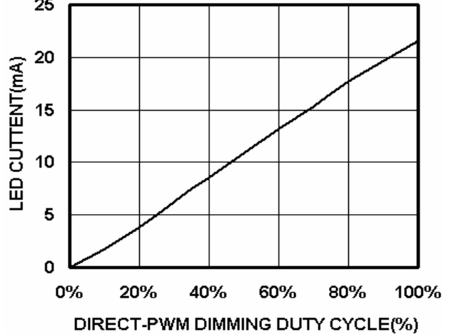
LED CURRENT vs DIRECT-PWM DIMMING DUTY CYCLE
