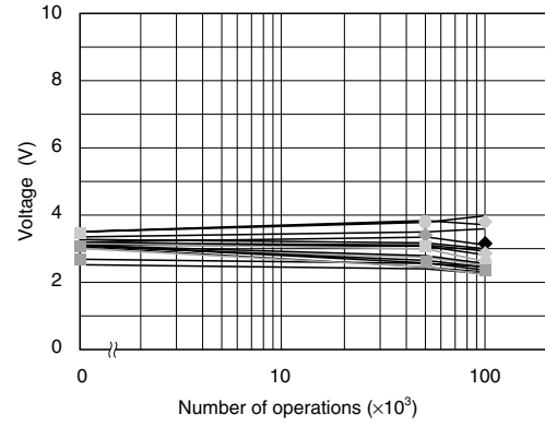
Release Voltage
