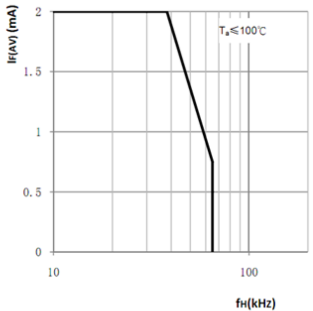
I_F (AV)-fH Curve
