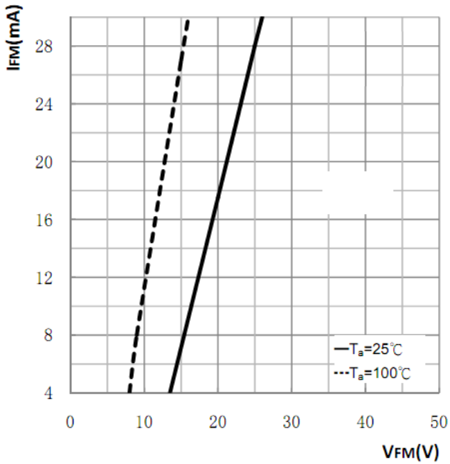
Forward Characteristics
