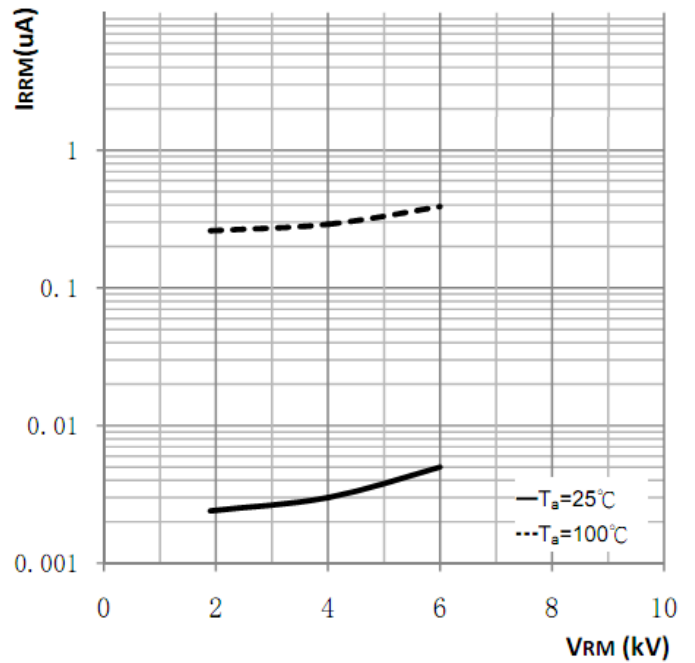
Reverse Characteristics
