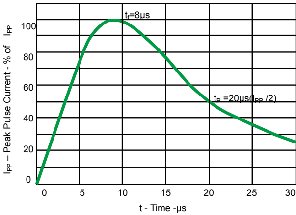
Fig 1. Pulse Waveform
