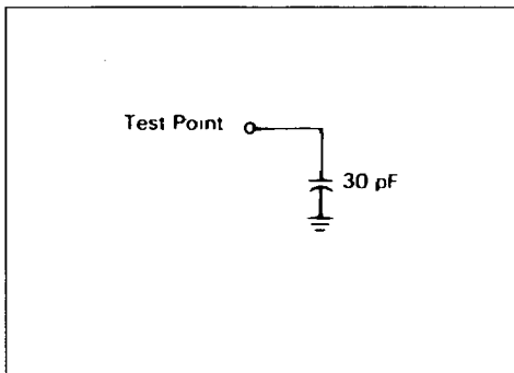
Figure 7 : CMOS Load.
