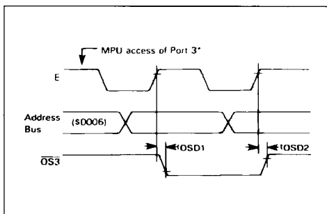
Figure 4 : Port 3 Output Strobe Timing (EF6801 single-chip Mode).
