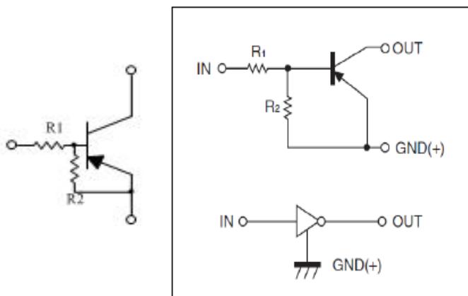
Equivalent Circuit
