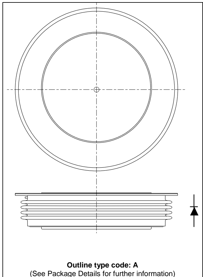
Fig. 1 Package outlines
