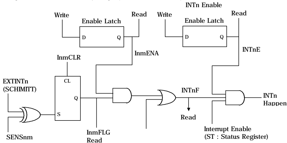
Figure 5-2. External Interrupt Logic (n = 1, 3 or 5 ; m = 0)
