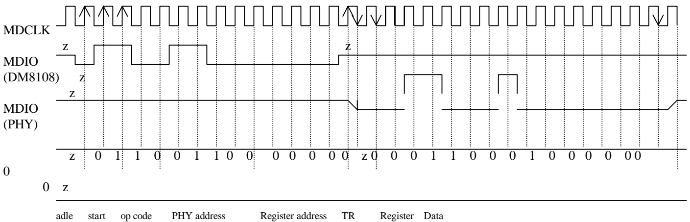
Figure Typical MDIO Read Operation
