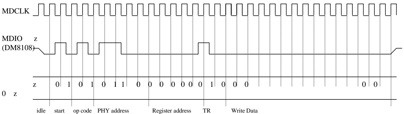
Figure Typical MDIO Write Operation
