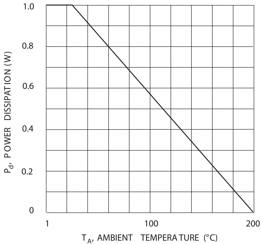
Fig. 1, Power Derating Curve
