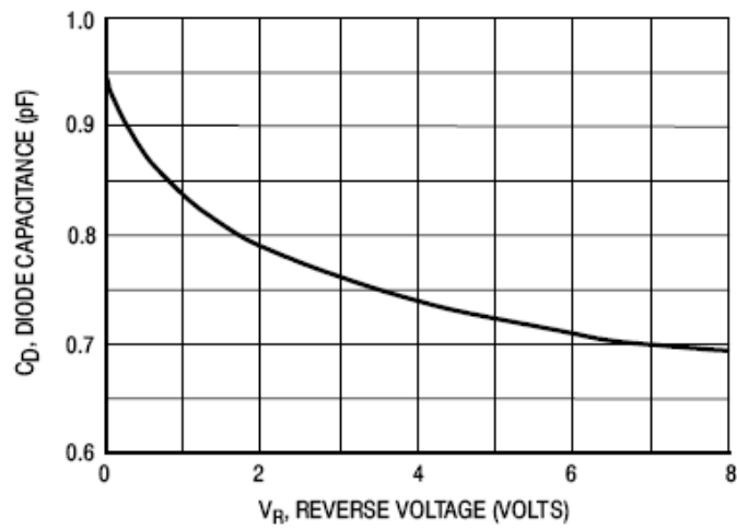
Figure 3. Diode Capacitance
