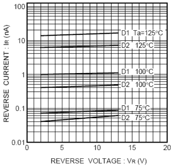
Fig.3 Reverse characteristics
