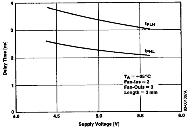
Delay Time vs Supply Voltage [NAND]
