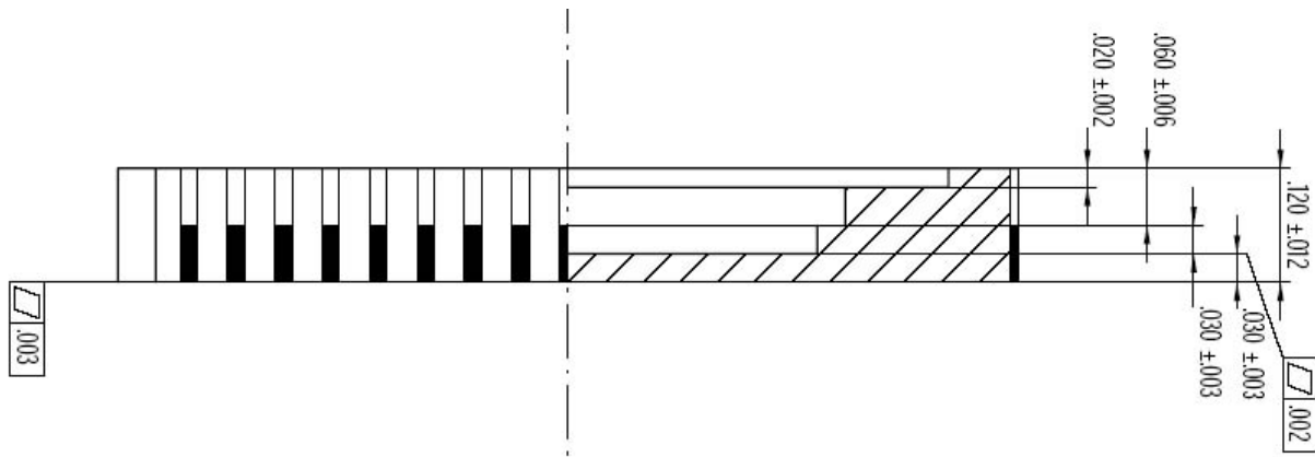
Figure 27. Package Side View (all dimensions in inch)
