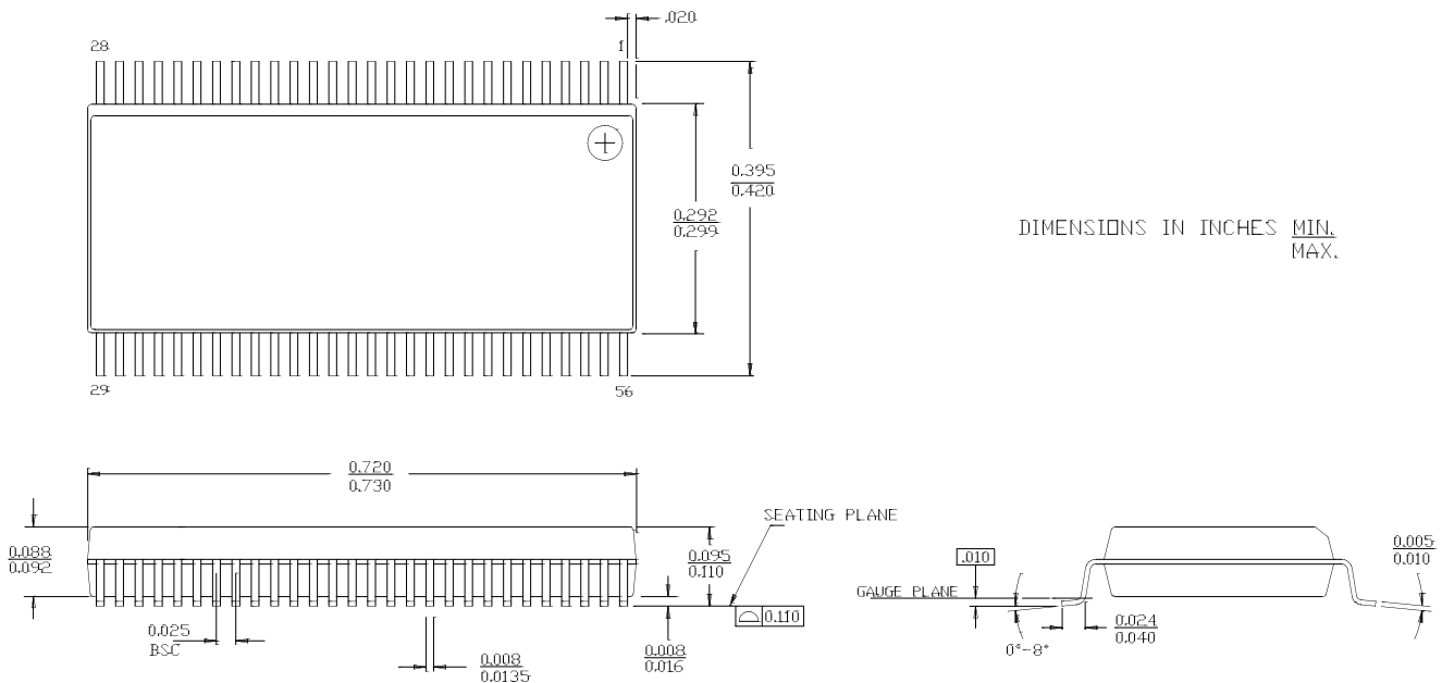
56-Lead Shrink Small Outline Package O56
