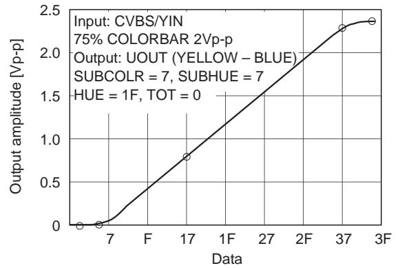
COLOR control characteristics
