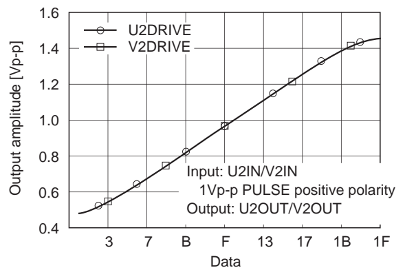
R2/V2DRIVE control characteristics
