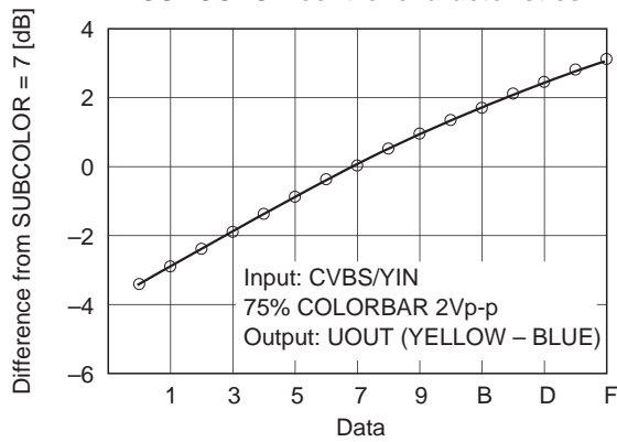
SUBCOLOR control characteristics
