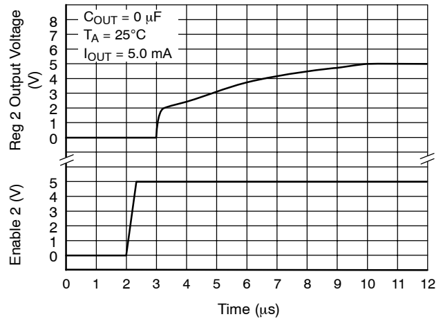
Figure 15. Regulator 2 Startup
