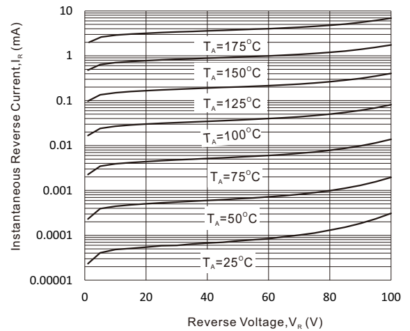
Fig. 2 - Reverse Characteristics
